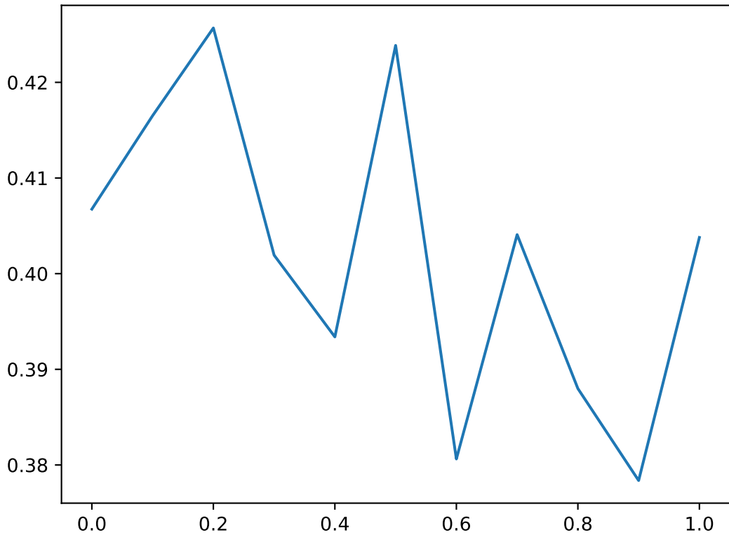
Average Ricci Curvature
